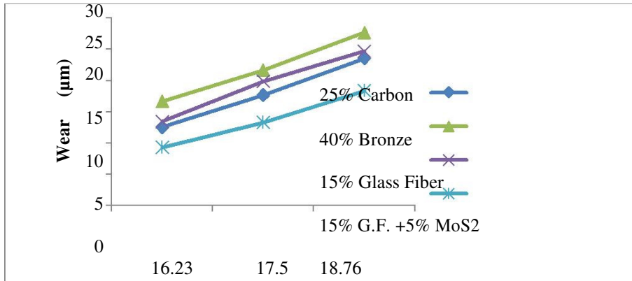
Fig.2 Wear Vs. Load for PTFE composites under dry condition.
