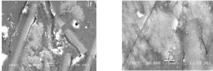
(a) (b) Fig. 4 SEM image of 15% Glass fiber + 5% MoS 2 filled PTFE sample before and after wear test
