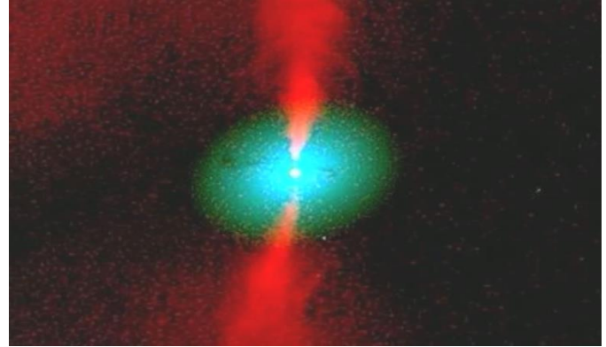
FIG.2. View of the M-84 galaxy in radio band
