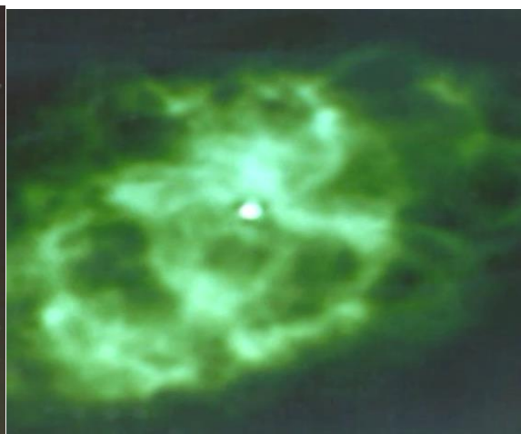
FIG.4. Pulsar(neutron Star). In radio band.
