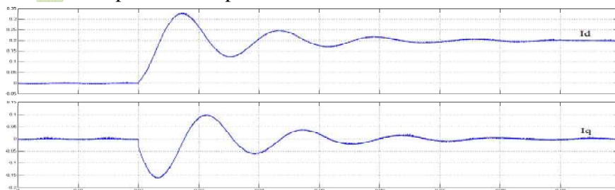
Figure 11: Id / Iq current component converter response during LG fault condition in phase A
