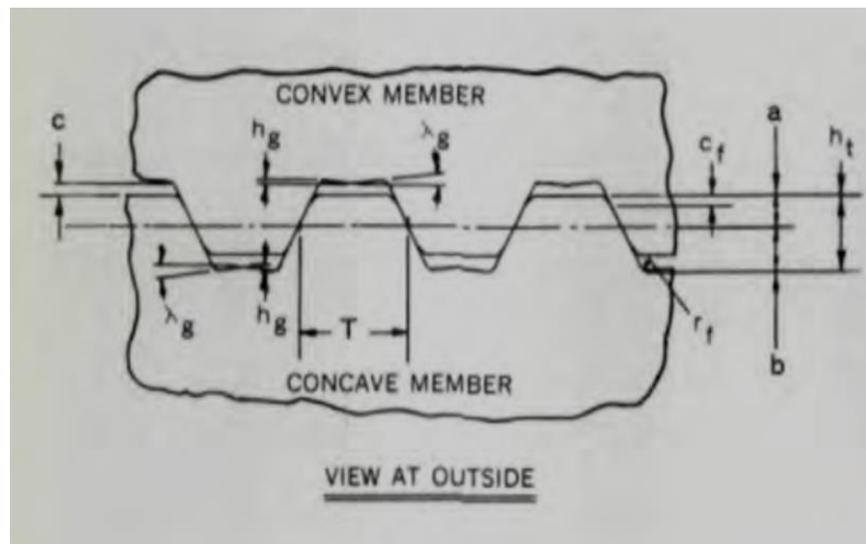
Fig : Fixed Curvic Coupling.
