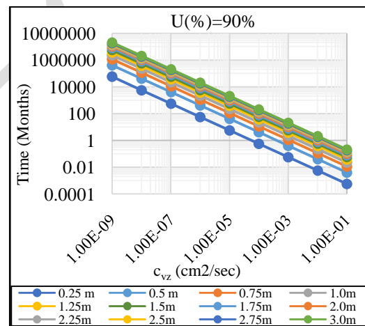
Figure 12: Variation of coefficient of consolidation with time for varying spacing, constant percent consolidation ( U\%=90\% )
