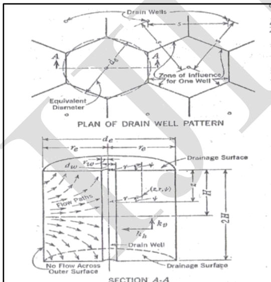
Figure 1: Plan of drain well pattern and fundamental concepts of flow within zone of influence of each well
