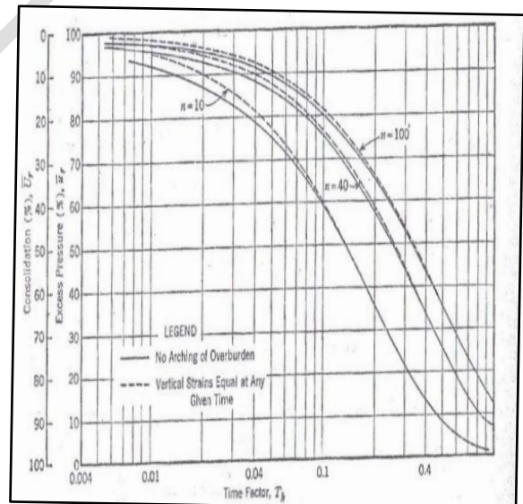
Figure 2: Average degree of consolidation for various values of 'n' under 'equal strain' condition at any given time
