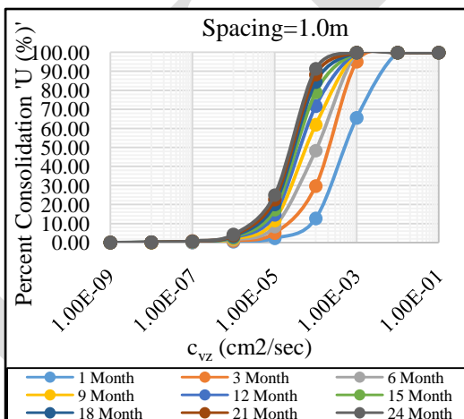
Figure 11: Variation of coefficient of consolidation with percent consolidation for varying time, constant spacing ( S=1.0\text{m} )
