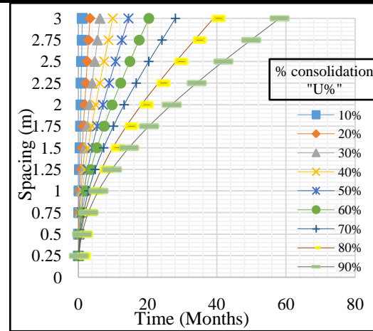
Figure 10: Variation of Spacing with Time for Varying Percent Consolidation ( U\% ) ( c_{vz}=4 \times 10^{-04} \text{ cm}^2/\text{sec} , c_{vr}=1.0c_{vz} )
