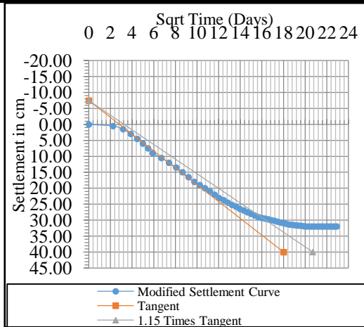
Figure 14: Modified settlement curve/ Taylor's Method (Sett. marker)(A-1)
