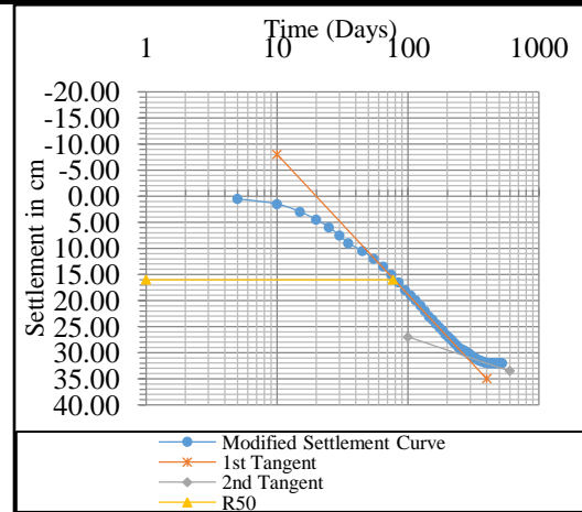
Figure 15: Casagrande's Method (Settlement Marker) (A-1)
