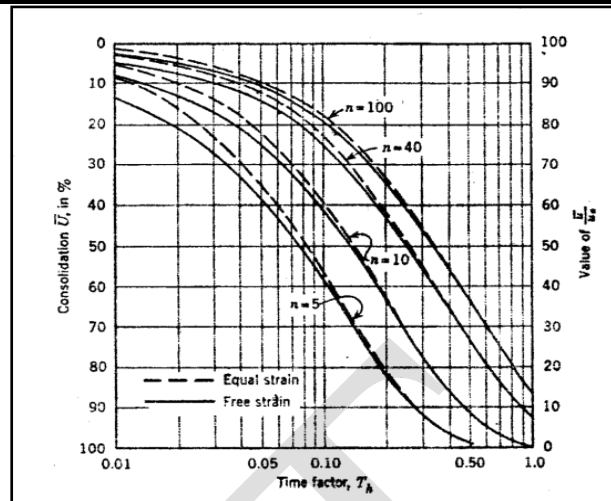
Figure 4: Comparison of equal strain and free strain
