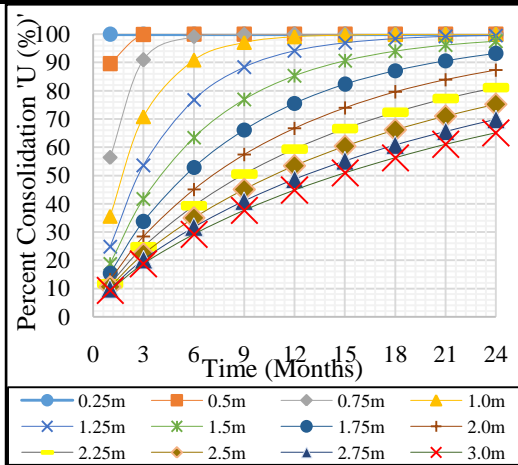
Figure 9: Variation of Percent Consolidation with Time for varying Spacing ( c_{vz}=4 \times 10^{-04} \text{ cm}^2/\text{sec} , c_{vr}=1.0c_{vz} )
