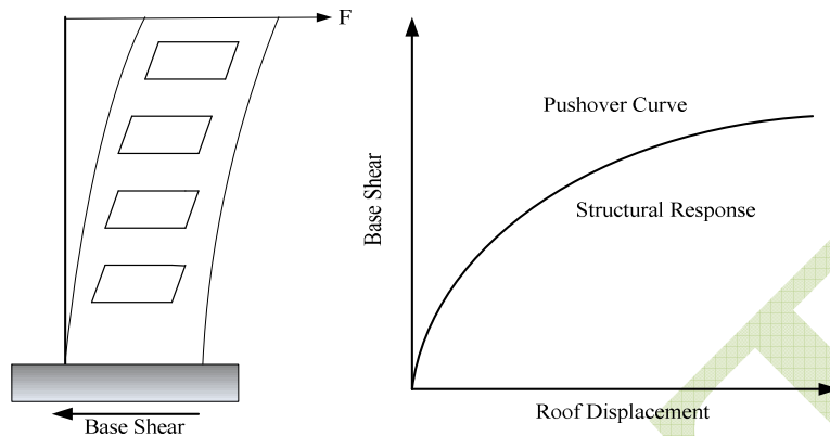
Fig. 2.1: (Pushover) Capacity Curve of the structure
