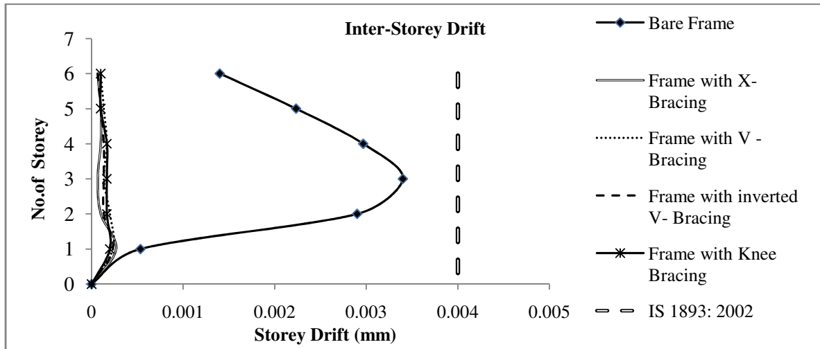
Fig.4.2: Inter storey drift ratio for steel bare frame with diff. bracing patterns in X- direction
