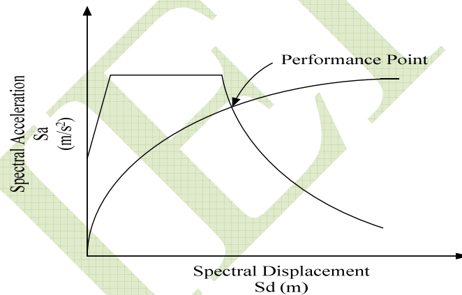
Fig. 2.4: Performance Point
