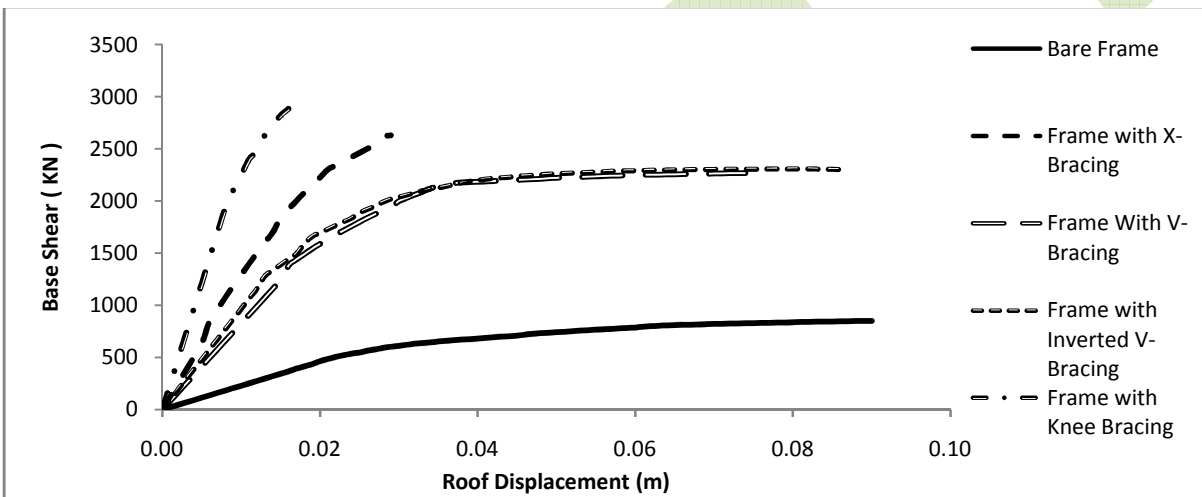
Fig.4.1: Pushover Curve for bare frame with diff. types of bracing patterns
