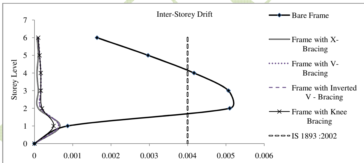
Fig.4.3: Inter storey drift ratio for steel bare frame with diff. bracing patterns in Y- direction
