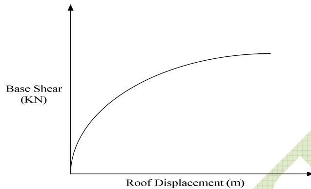
Fig.2.3: Capacity Curve
