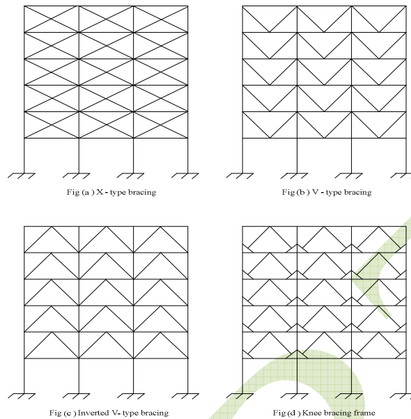
Fig.3.1: Diff. types of bracing configurations
