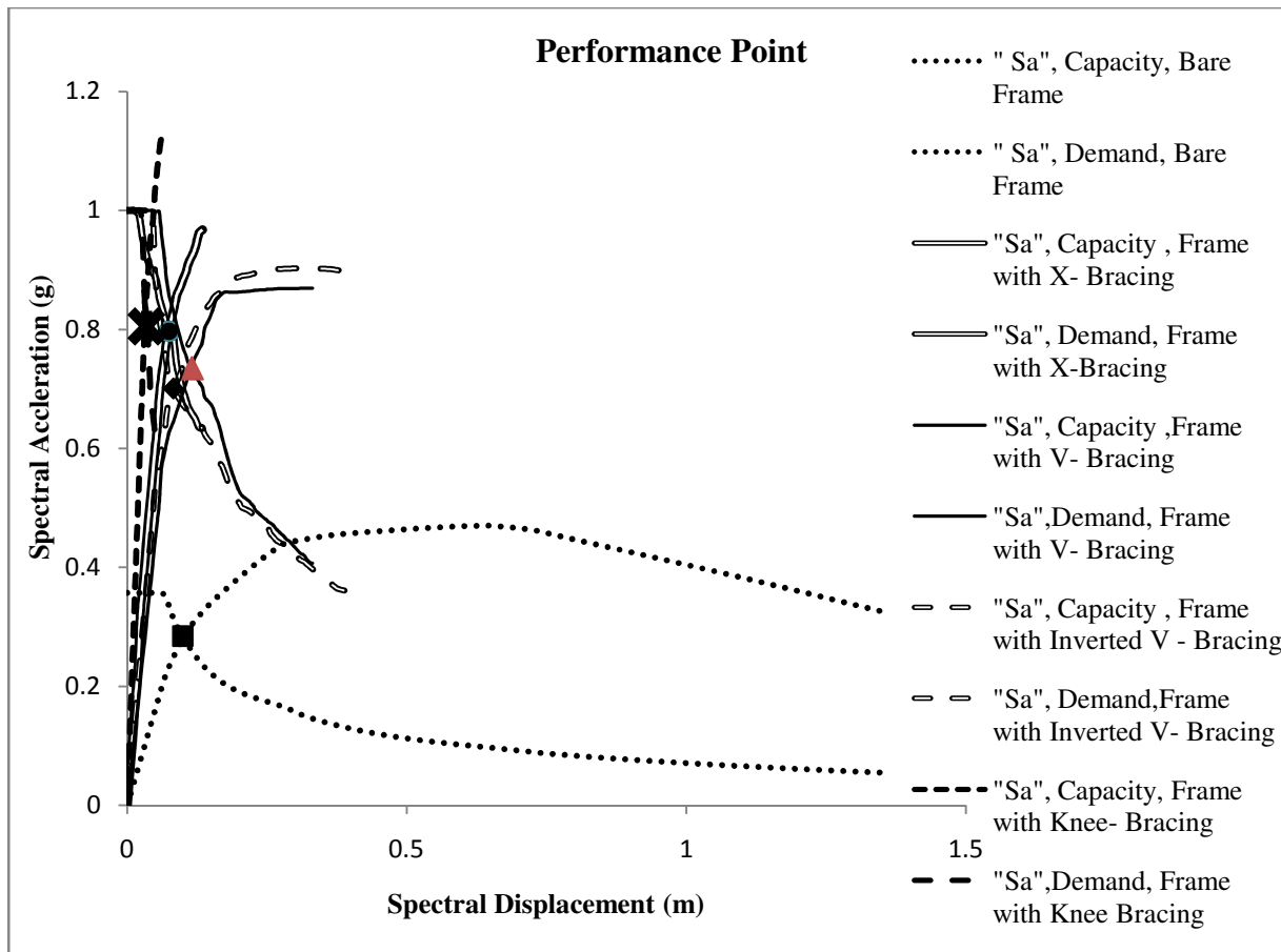
Fig.4.4: Performance point for steel bare frame with diff. bracing patterns
