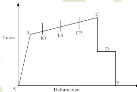
Fig.2.5: Force Vs Deformation Curve
