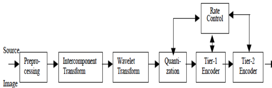
Figure 3 Structure of adaptive JPEG2000 compression.
