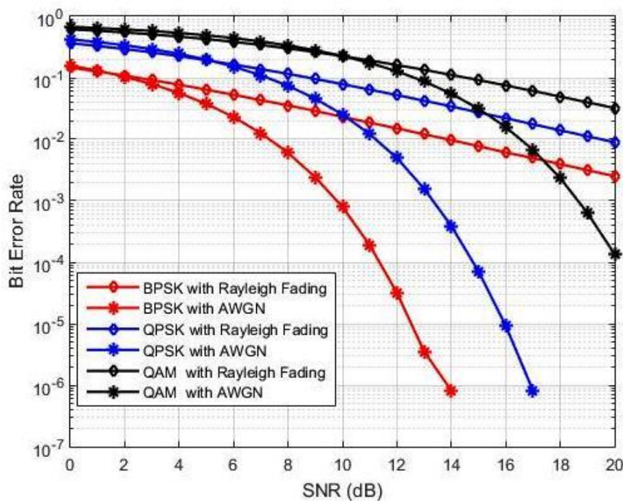
Figure 4 Bit error rate vs. SNR.
