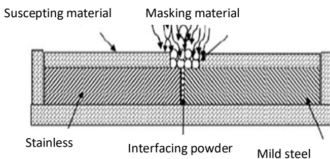
Figure 1.3: Principle of microwave joining of two materials
