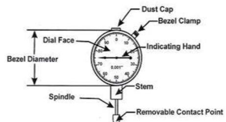
Fig 3: Specifications of dial gauge [5]
