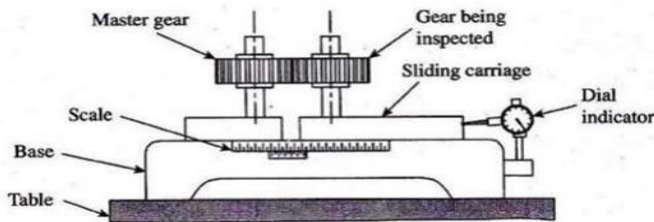
Fig. 1: Experimental setup of Parkinson's Gear Tester [1]
