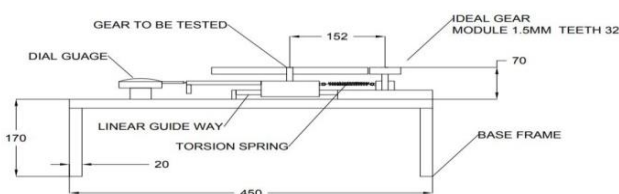
Fig. 2: Line diagram of Parkinson's Gear Tester [5]
