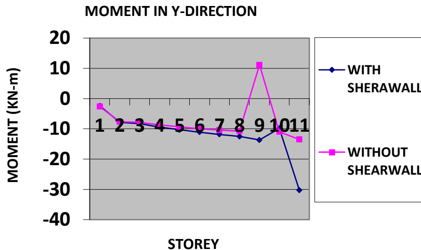
Graph – 5: Comparison of Moment along Y-direction in frame system with and without shearwall location
