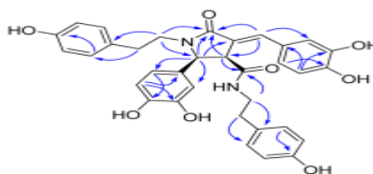
Figure 3. Key HMBC correlations for compound.
