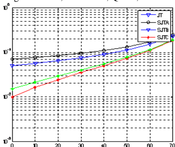
Figure.5: BER versus K performance of conventional JT and SJT in a Rayleigh channel of P = 3 for \text{SNR} = 7 dB; L = 16 ; orthogonal codes; and BPSK, QPSK, and 8PSK modulation
