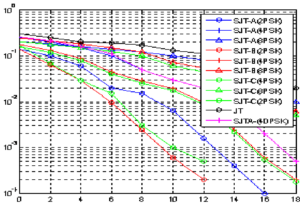
Figure.3:BER versus SNR performance of conventional JT and the three proposed SJT precoding methods in a Rayleigh fading channel of P = 3 paths for K = 5 ; L = 16 ; orthogonal codes; and BPSK, QPSK, and 8PSK modulation.
