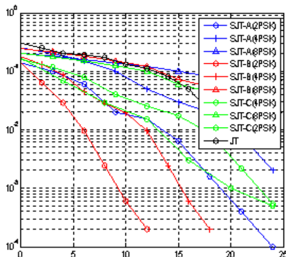
Figure.4: BER versus SNR performance of conventional JT and SJT in a Rayleigh fading channel of P = 11 for K = 8 users with unequal powers; L = 16 ; orthogonal codes; and BPSK, QPSK, and 8PSK modulation.
