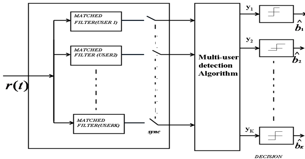
Figure.1: A typical multi-user detector
