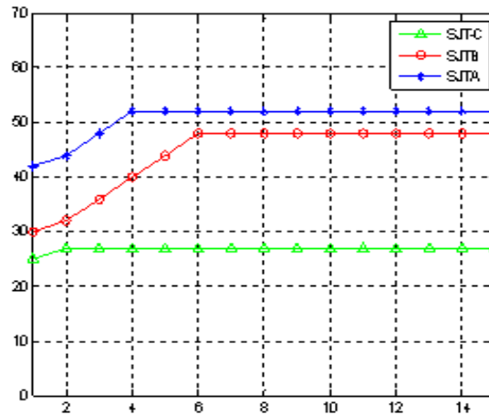
Figure.7: Decorrelating complexity of the three proposed SJT techniques for L = 16 , P = 11 , BPSK modulation, and SNR = 7 dB.
