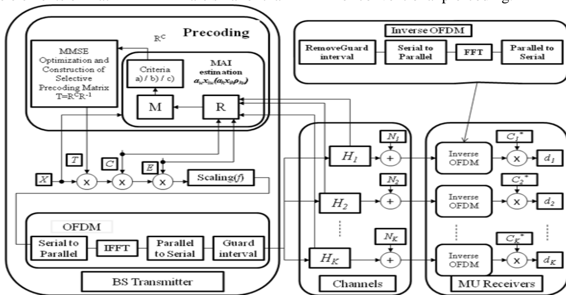
Figure.2: The proposed selective pre-coding in the MC-CDMA downlink
