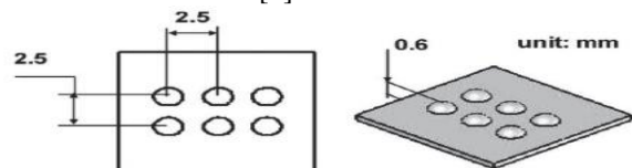
Fig. 2 - International building standard for a Braille cell
