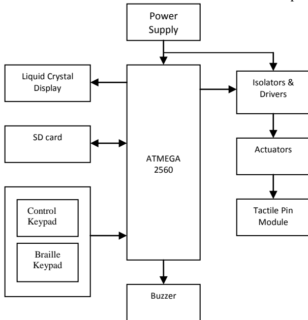
Fig. 5-Block Diagram
