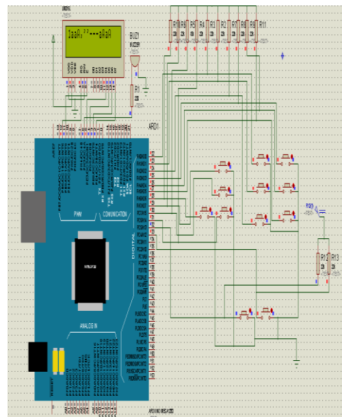
Fig. 6-Simulation diagram on proteus 7.8
